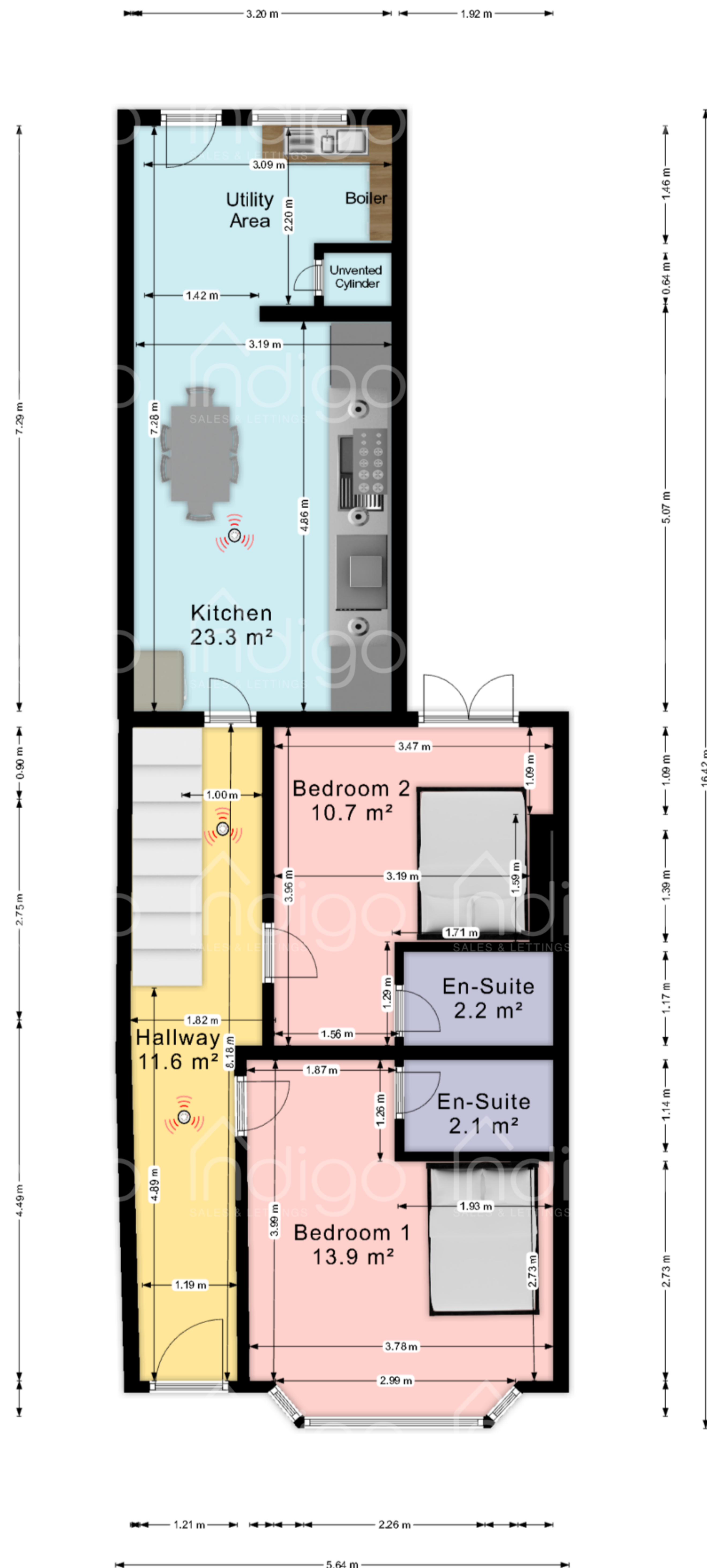
99 London Road - Ground Floor INDIGO Sales & Lettings - 01782 585041 The floor-plan is provided as a guide only & should be used for illustration although accurate. We accept no responsibility for any inaccuracies contained within the drawing.
